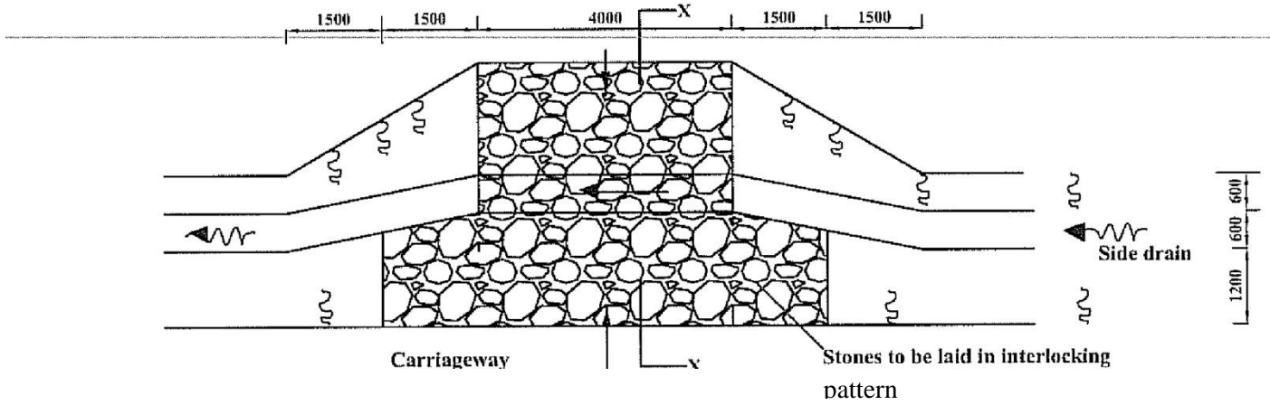
FIGURE C18-ACCESS DRIFT
