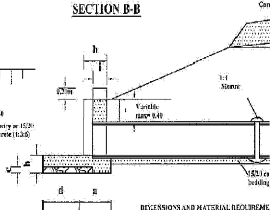
DIMENSIONS AND MATERIAL REQUIREMENTS
