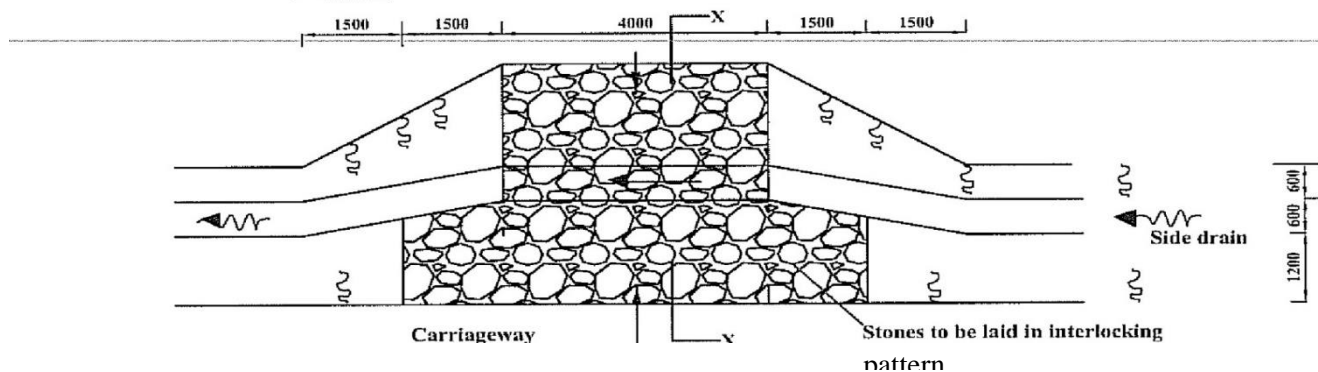
FIGURE C18-ACCESS DRIFT PLAN
