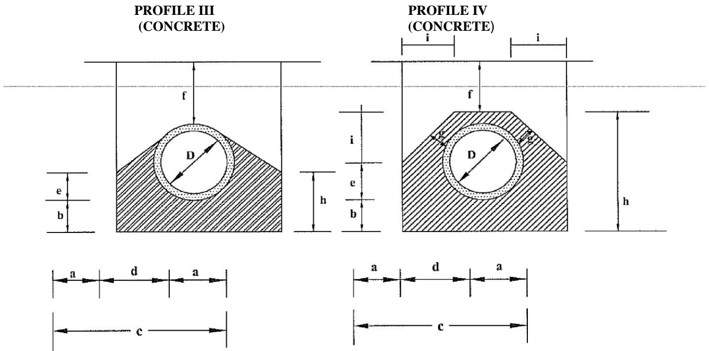
FIGURE C17-BEDDING AND SORROUND PROFILE TYPES III & IV
