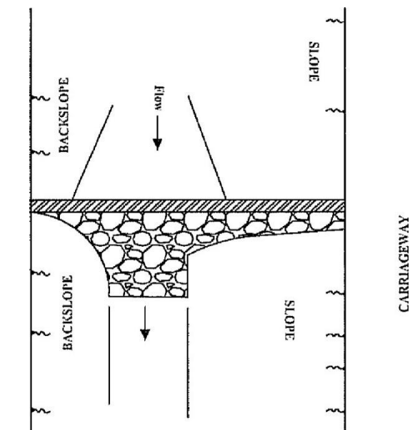
PLAN OF DRAIN WITH SCOUR CHECKS
