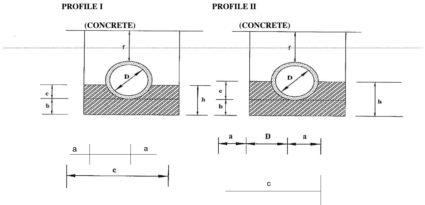
FIGURE C16-BEDDING AND HAUNCH PROFILE TYPES I & II
