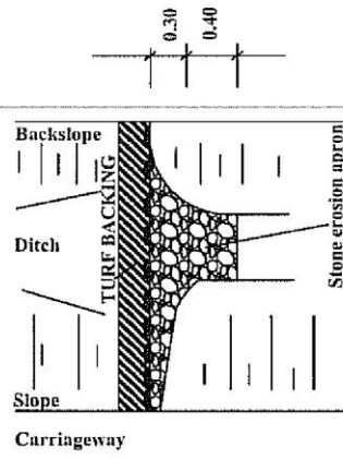
FIGURE C8-DIMENSIONS OF SCOUR CHECKS FOR STANDARD DRAIN
