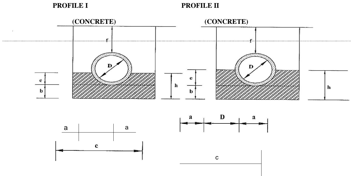
FIGURE C16-BEDDING AND HAUNCH PROFILE TYPES I & II
