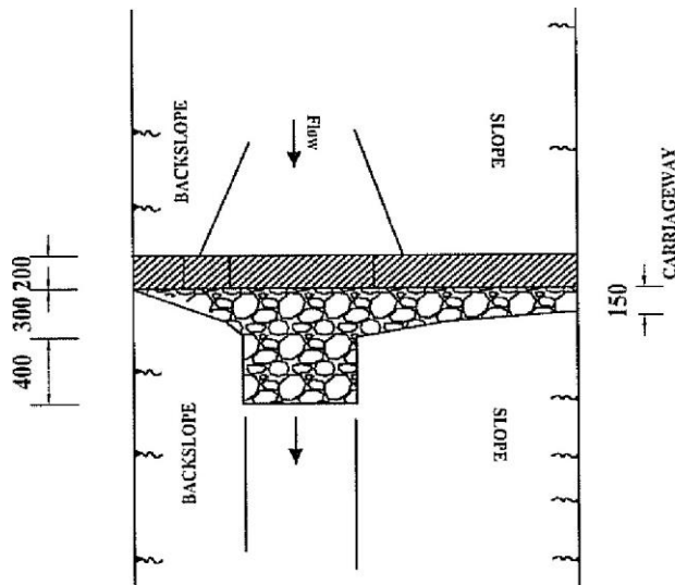
PLAN OF DRAIN WITH SCOUR CHECK
