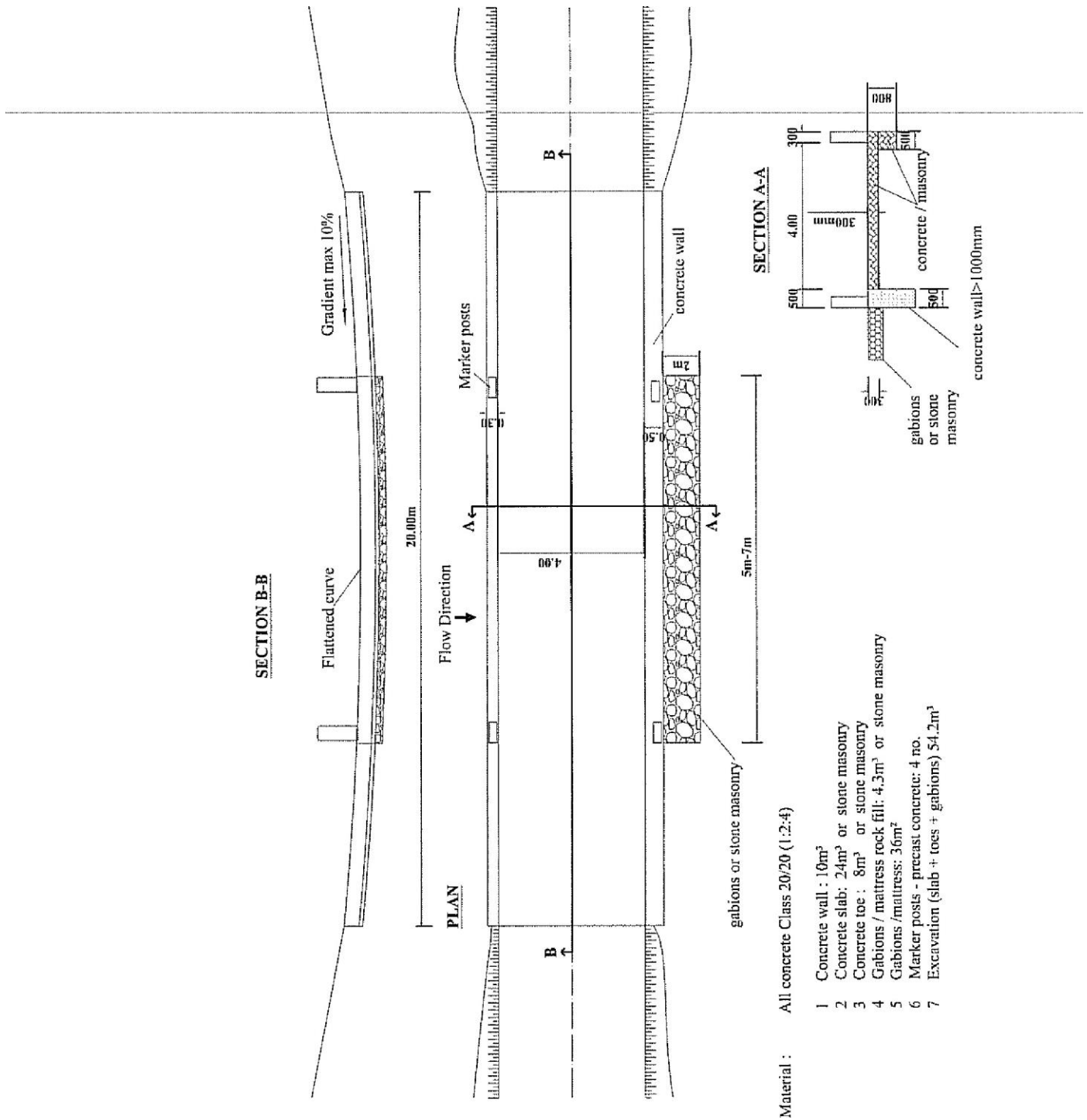
FIGURE C19-LEVEL DRIFT
