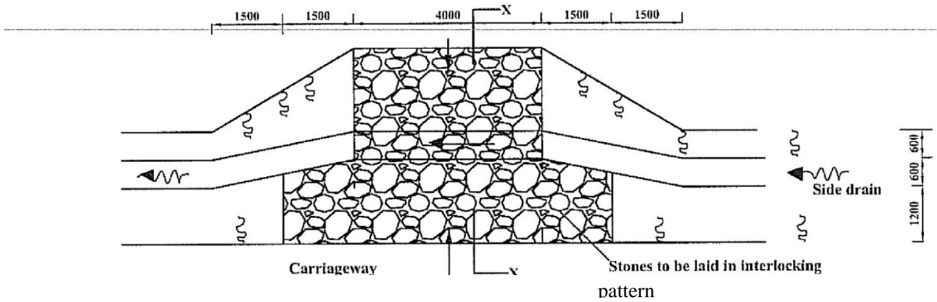
FIGURE C18-ACCESS DRIFT PLAN
