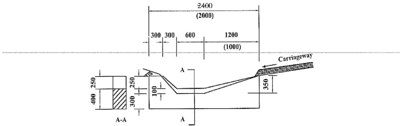
FIGURE C9a-MASONRY SCOUR CHECKS
