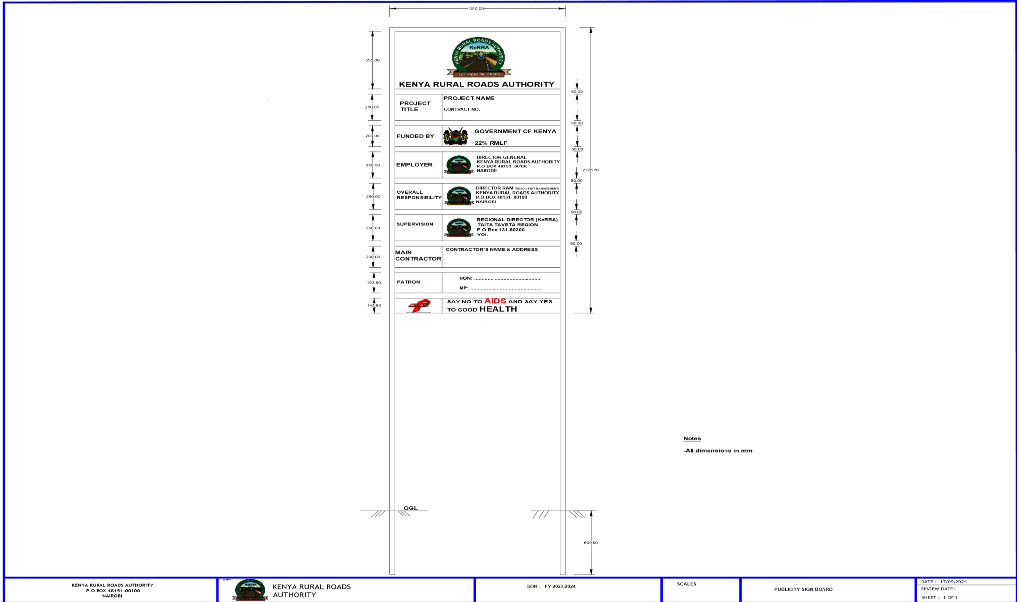
FIGURE C.18: PUBLICITY SIGNBOARD
