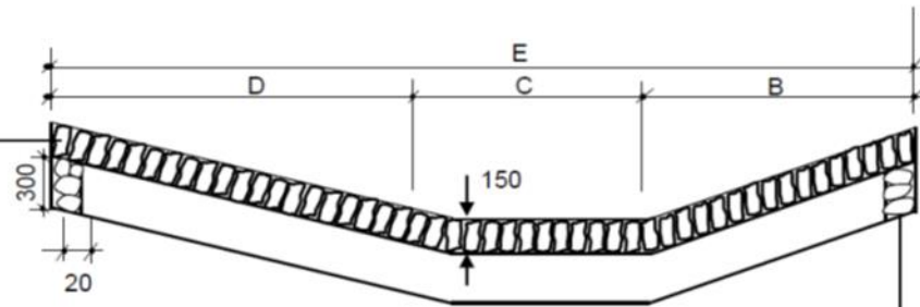
X-SECTION X-X
