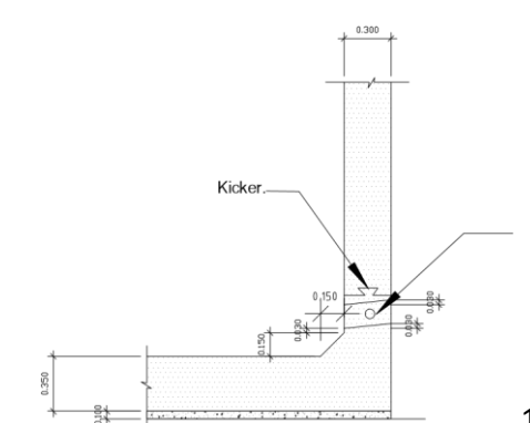
KICKER AND WEEPHOLE DETAIL. 1:25 DIMENSIONS:
