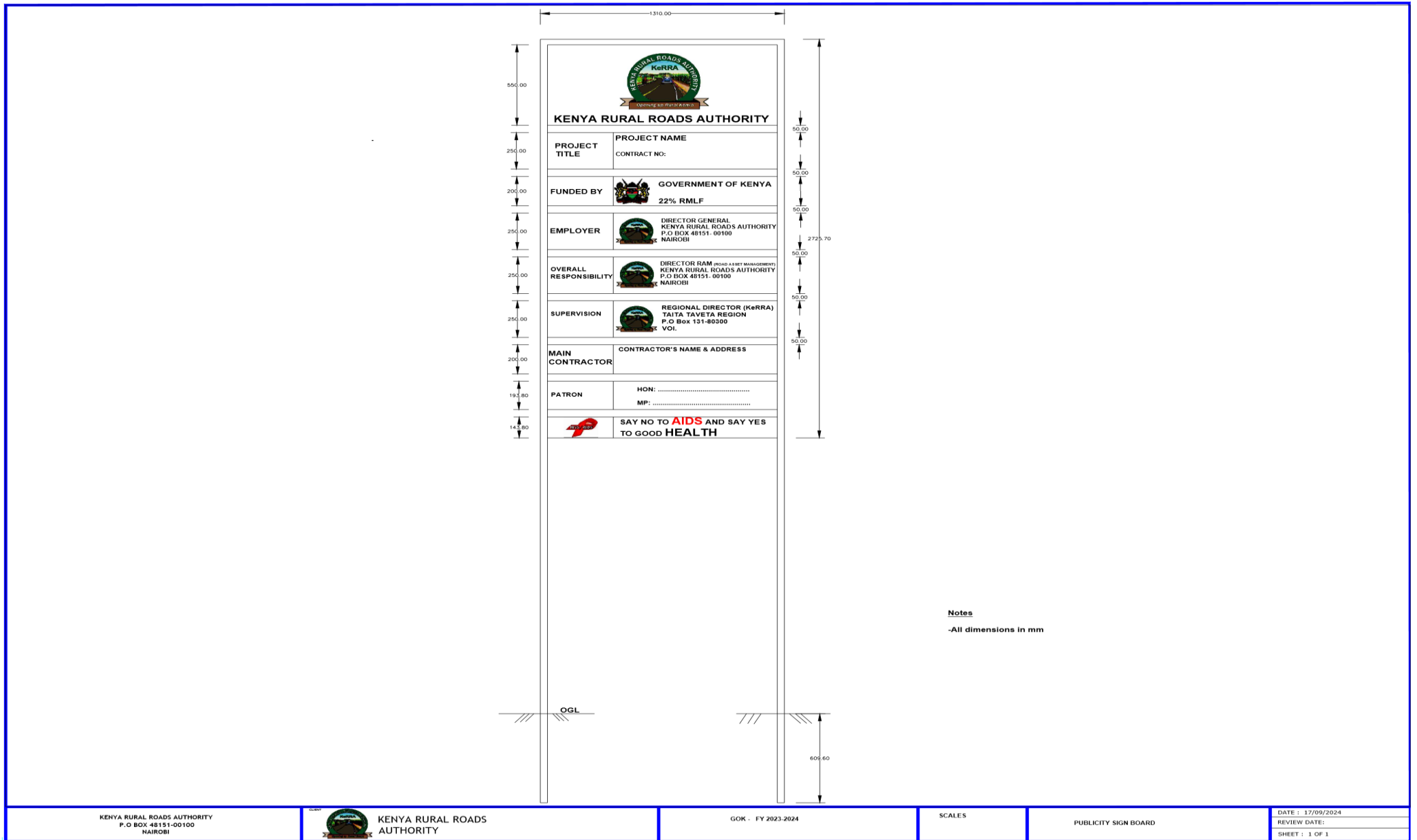
FIGURE C.17: PUBLICITY SIGNBOARD
