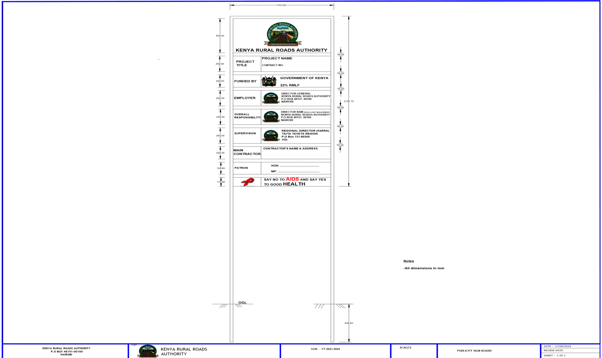
FIGURE C.17: PUBLICITY SIGNBOARD
