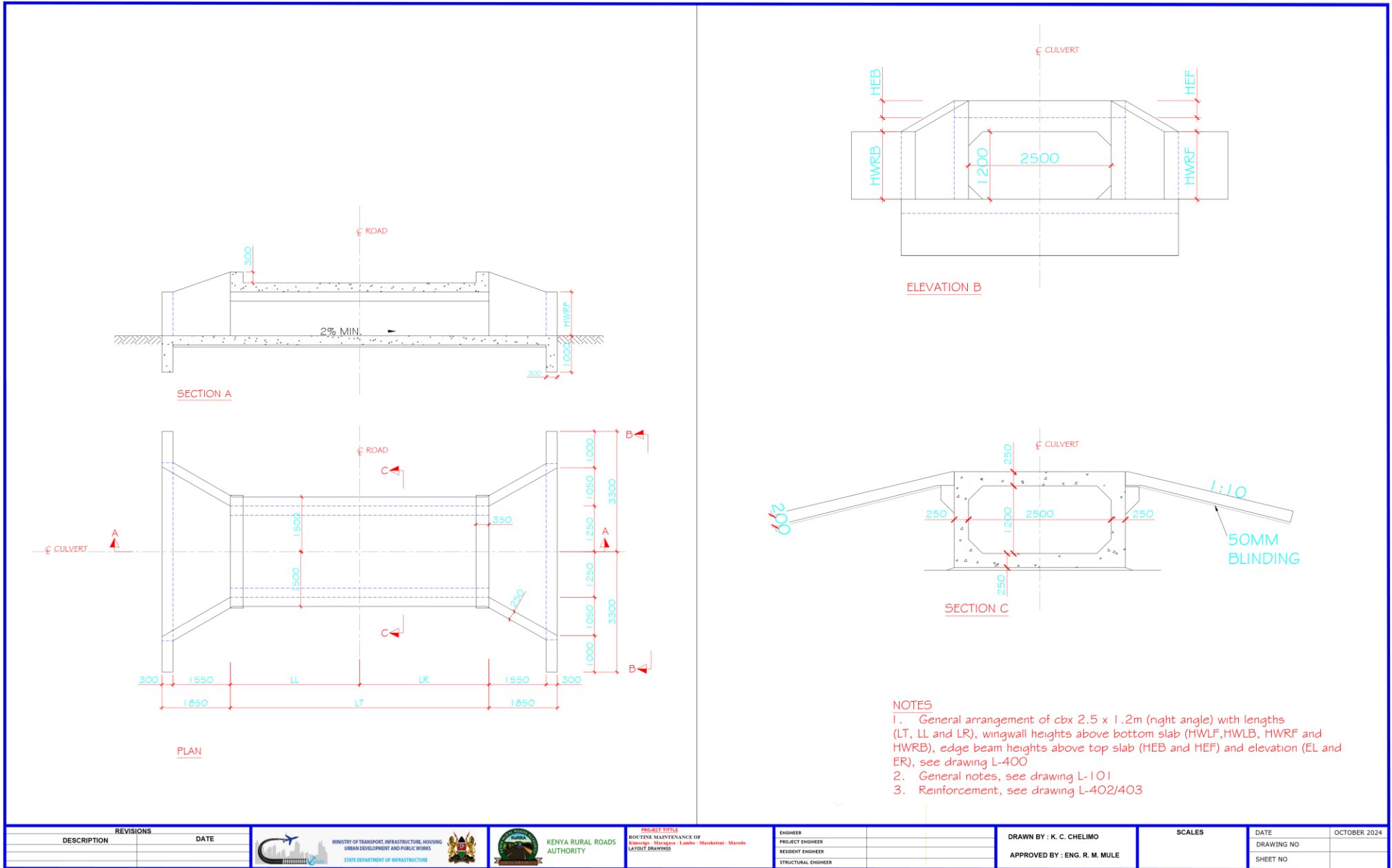
FIGURE C.17: 2.5x1.2m BOX CULVERT LAYOUT
