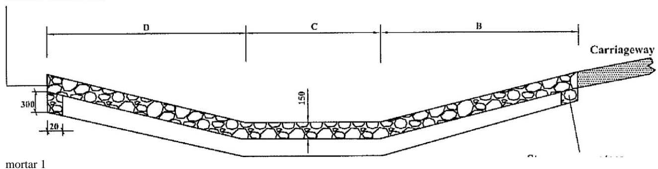
SECTION X-X
