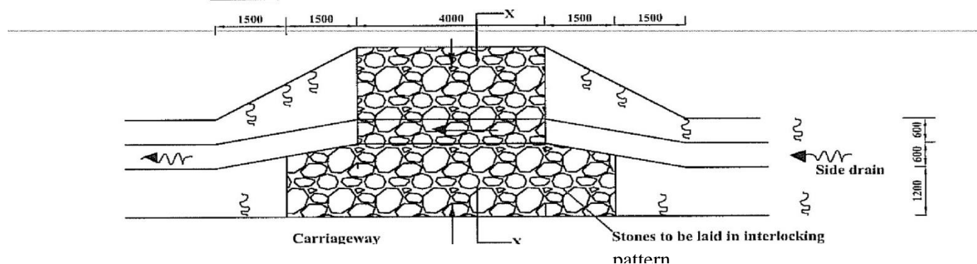
FIGURE C18-ACCESS DRIFT PLAN
