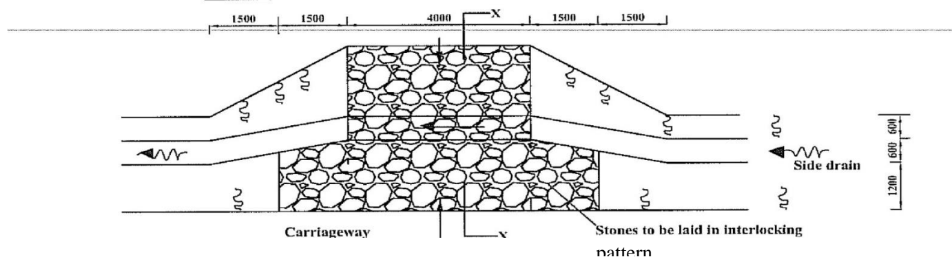
FIGURE C18-ACCESS DRIFT PLAN
