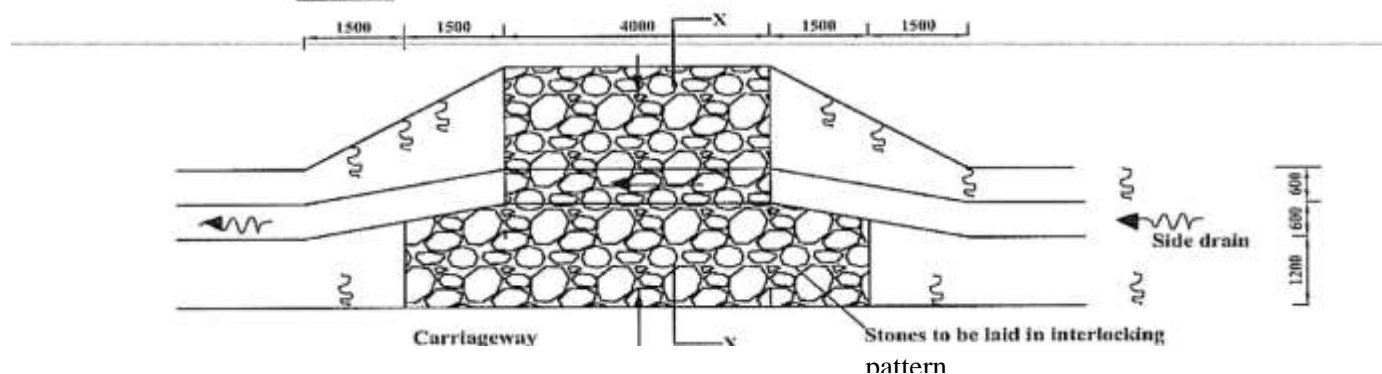
FIGURE C18-ACCESS DRIFT
