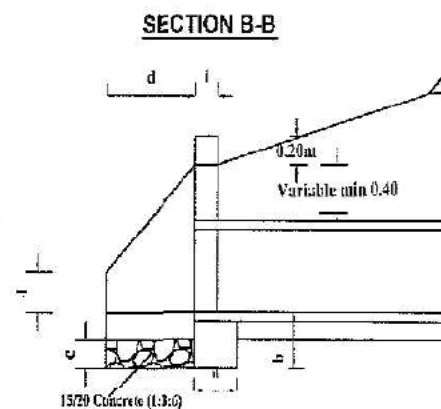
PIPE DIAMETER IN (IN) TYPE A (CONCRETE BLOCKS) 450 600 900 DIMENSION UNIT a FOUNDATION m 0.30 0.36 b FOUNDATION m 0.30 0.36 c APRON m 1.34 1.49 d APRON m 0.40 0.50 e APRON m 0.34 0.30 f WINGWALLS m 0.20 0.20 g WINGWALLS m 0.10 0.10 h HEADWALLS m 0.69 0.69 i HEADWALLS m 0.20 0.20 k HEADWALLS m 0.65 0.80 l HEADWALLS m 0.40 0.40 MATERIAL REQUIREMENT FOUNDATION (concrete blocks) 0.18 0.20 HEADWINGWALLS (Concrete/Masonry) 0.28 0.32 APRON (concrete) 0.12 0.14
