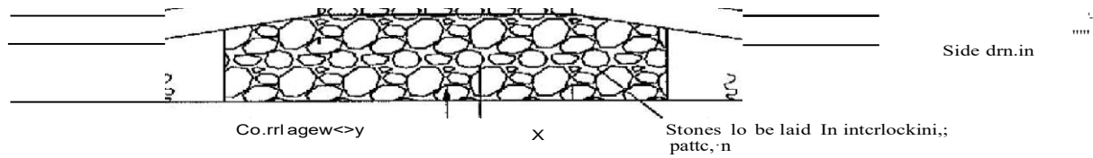
1 Stone Grouted Stone Pitching (Cement mortar 1:4)
