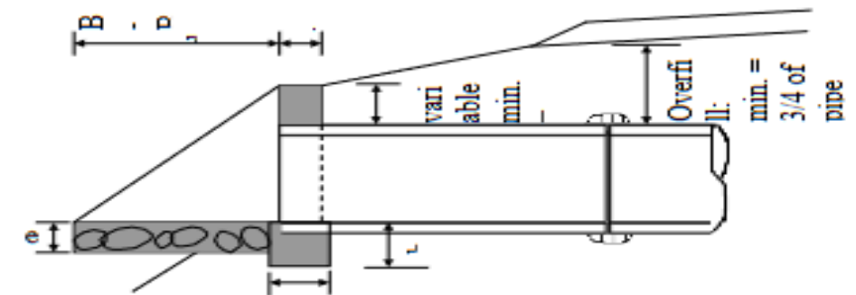
Concrete 1:2:4 DIMENSIONS AND MATERIAL REQUIREMENTS
