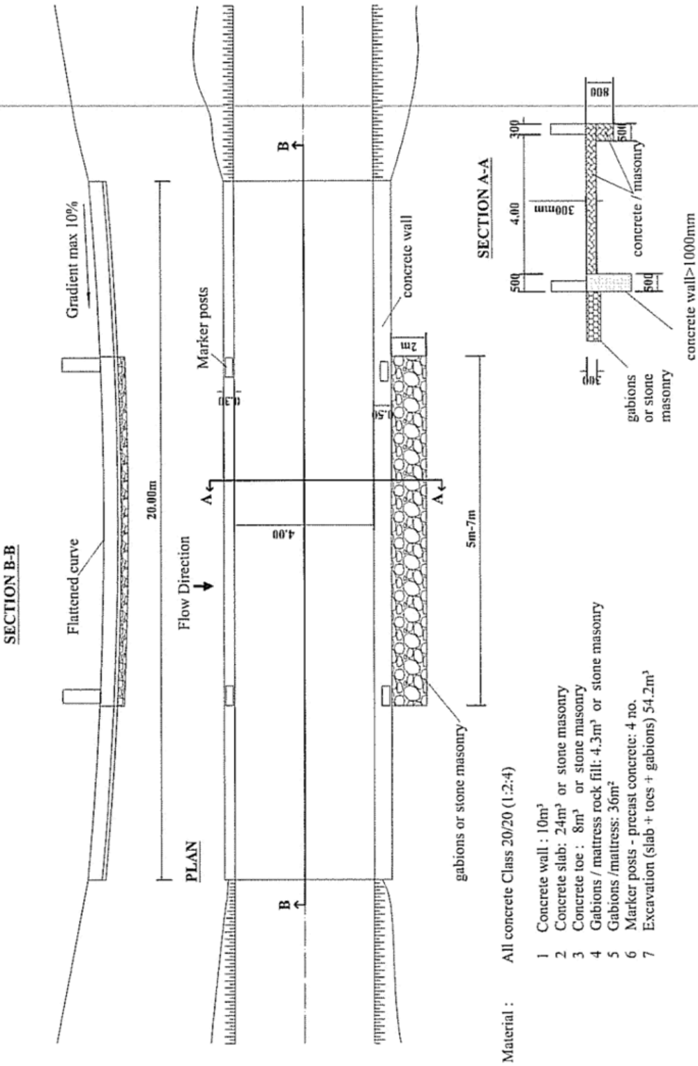
FIGURE C19-LEVEL DRIFT
