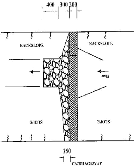
PLAN OF BRAIN WITH SCOUR CHECK
