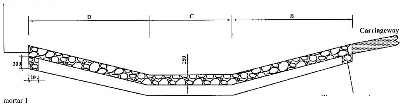
SECTION X-X
