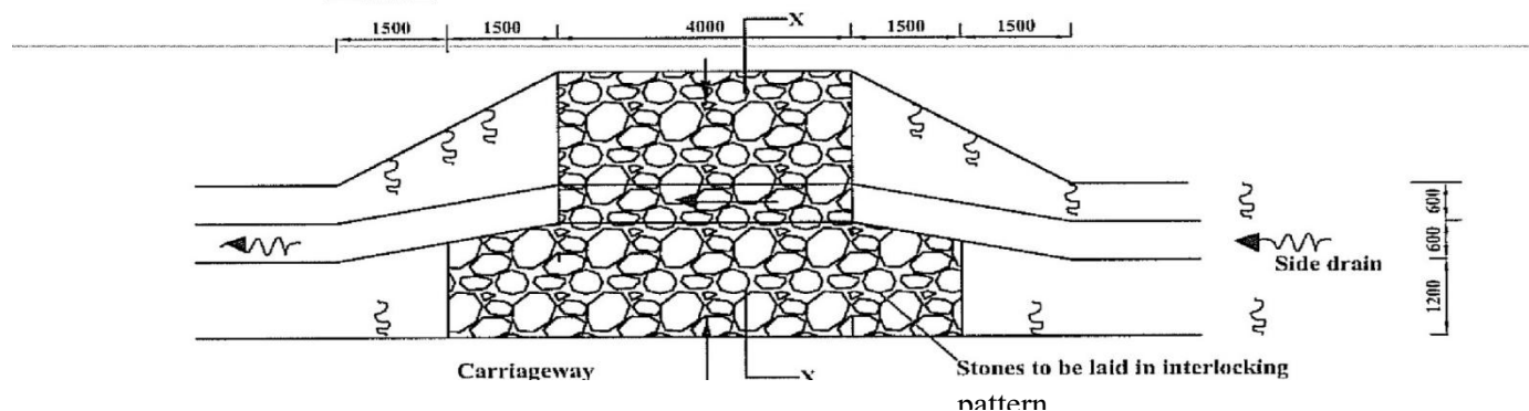
FIGURE C18-ACCESS DRIFT PLAN
