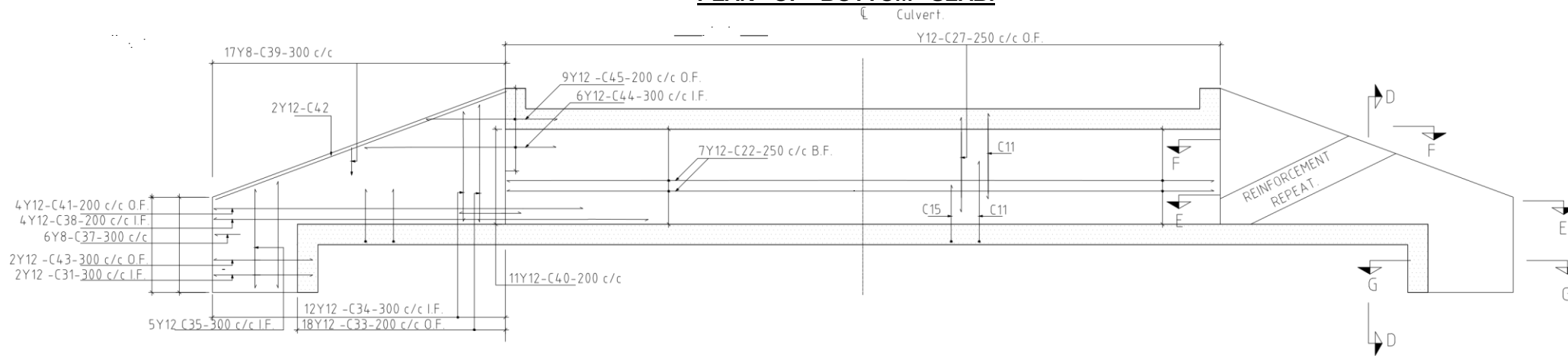
ELEVATION OF WALL & WINGWALL.
