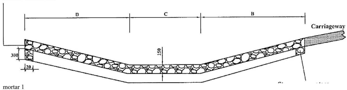
SECTION X-X
