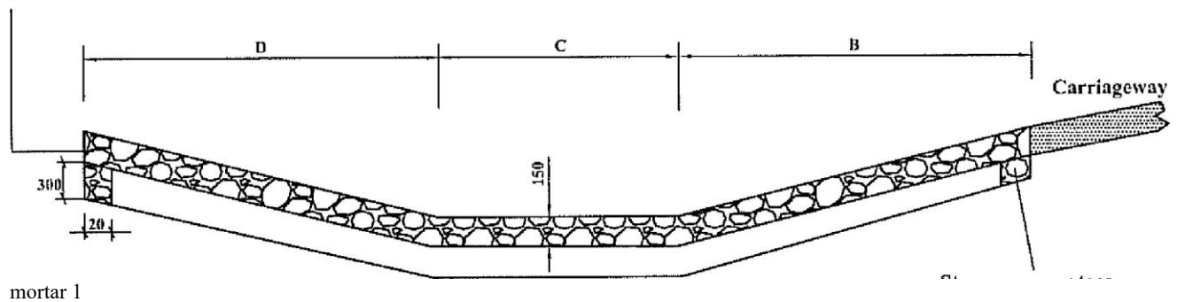
SECTION X-X
