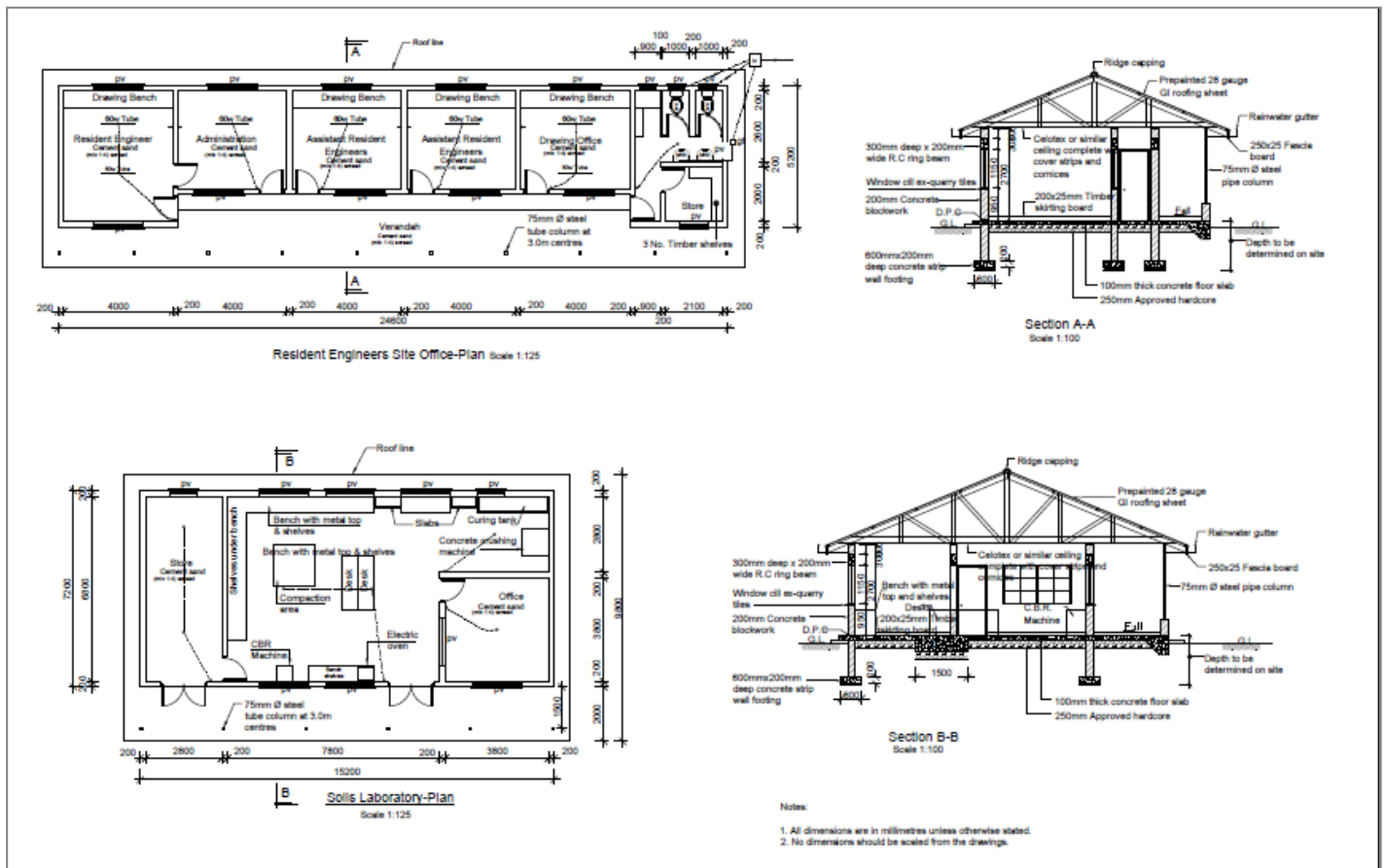
RE's Office and Site Laboratory Drawings
