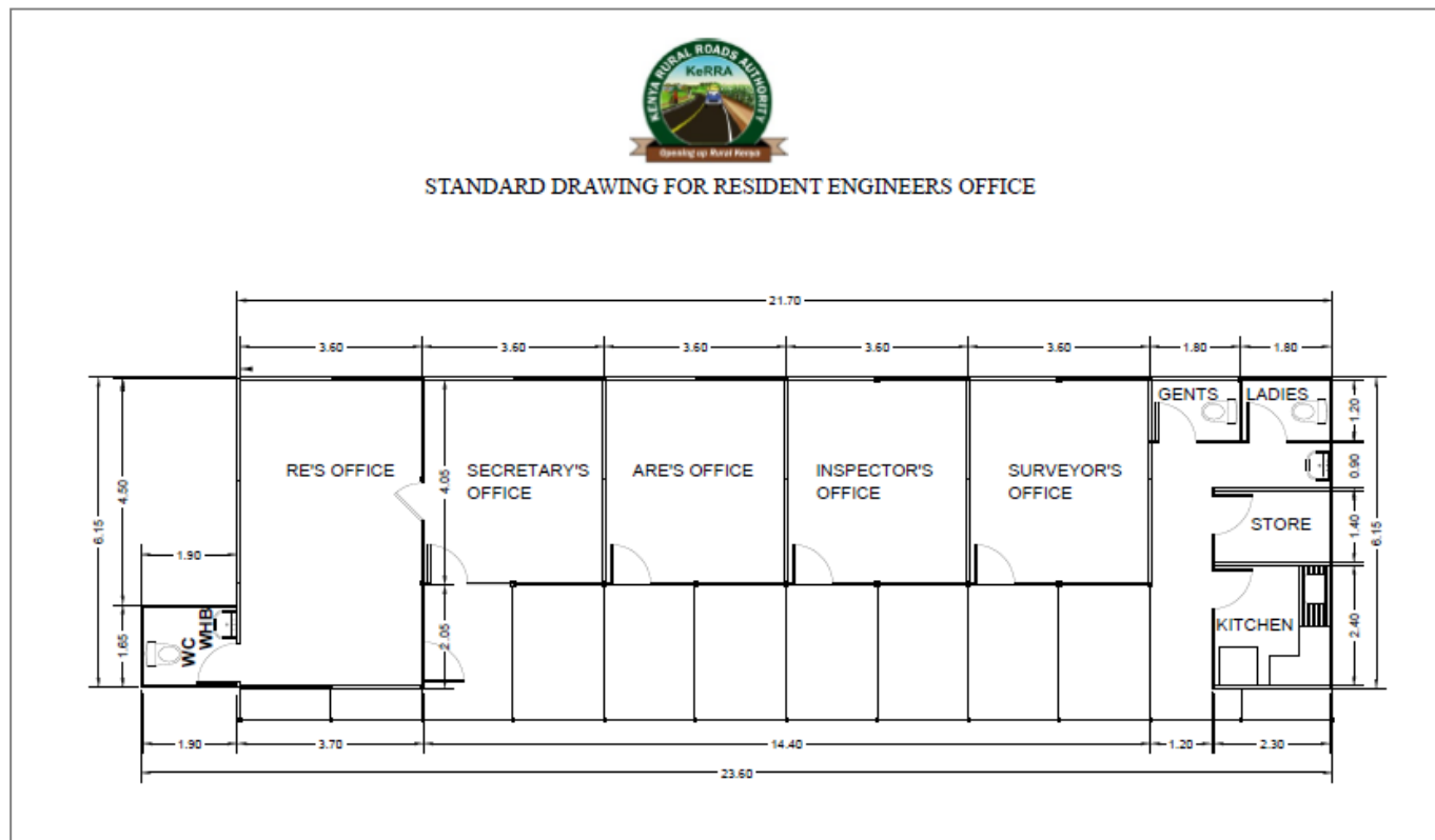
RE's Office Plan
