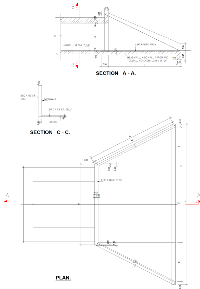
Fig. C.8 Standard pipe culvert Dimensions (900mm & 600mm Diameter)
