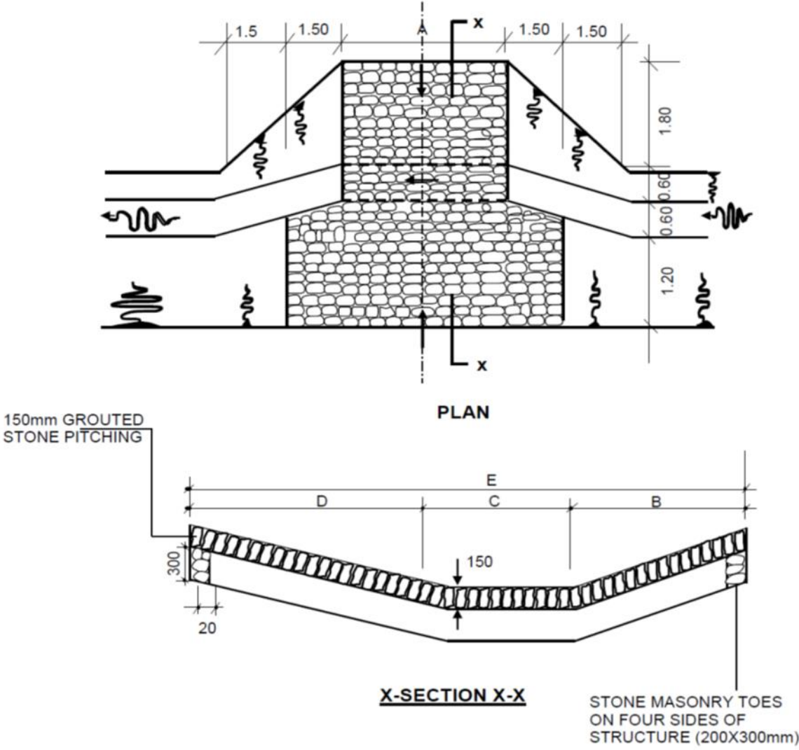
FIGURE C.15 ACCESS DRIFT
