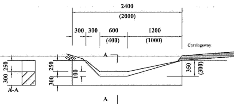
FIGURE C9b- CONCRETE SCOUR CHECKS
