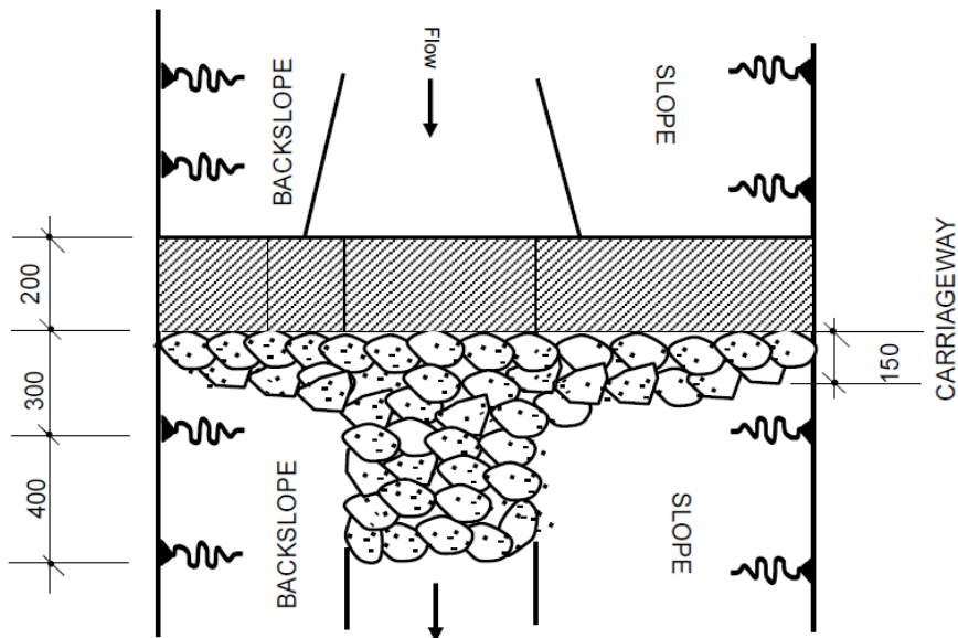
PLAN OF DRAIN WITH EROSION CHECKS
