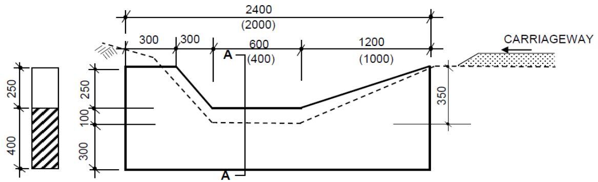
A SECTION OF MASONRY SCOUR CHECKS
