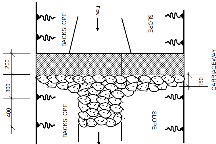
A SECTION OF MASONRY SCOUR CHECKS
