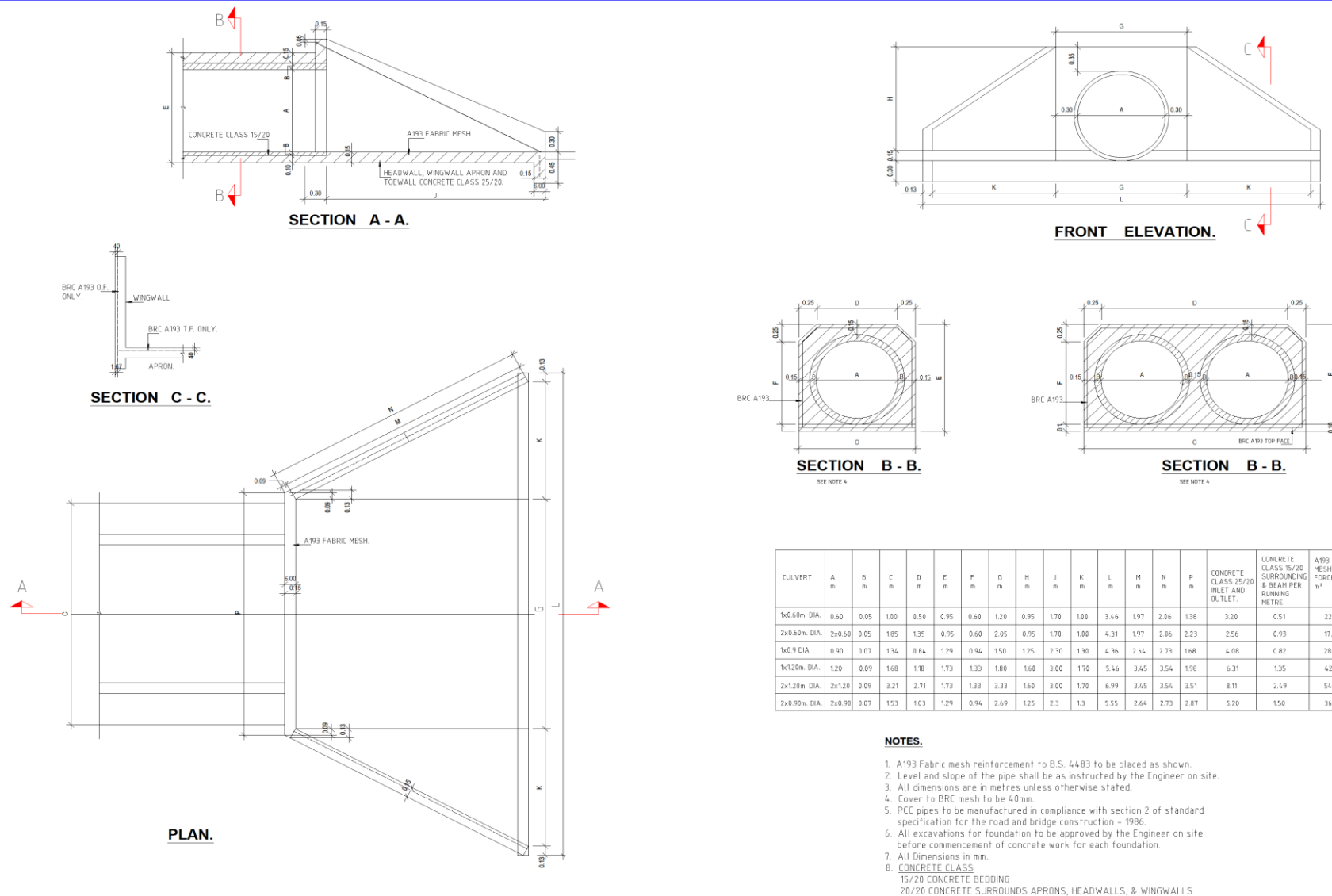
Fig. C.8 Standard pipe culvert Dimensions (900mm & 600mm Diameter)
