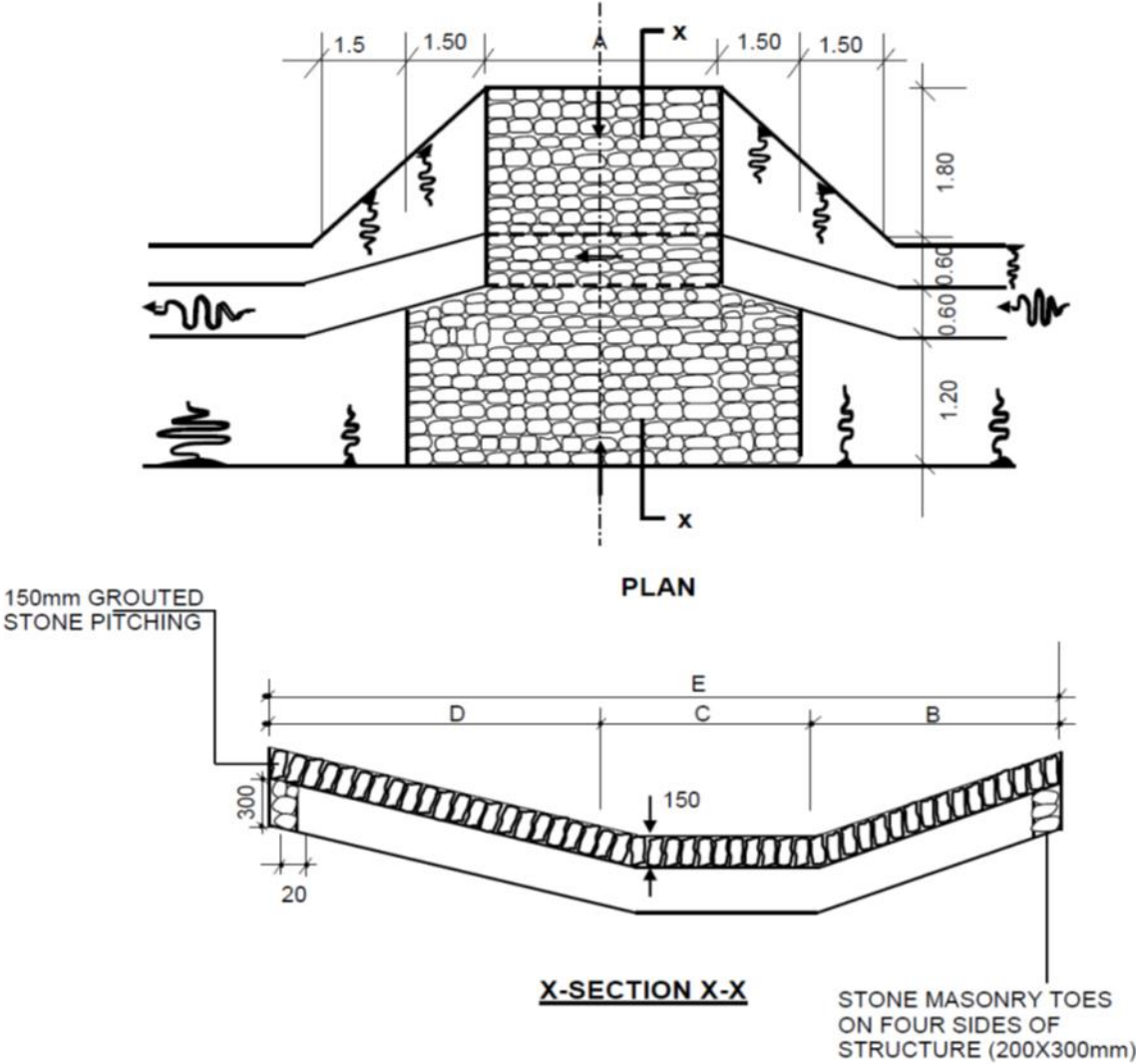
FIGURE C.15 ACCESS DRIFT
