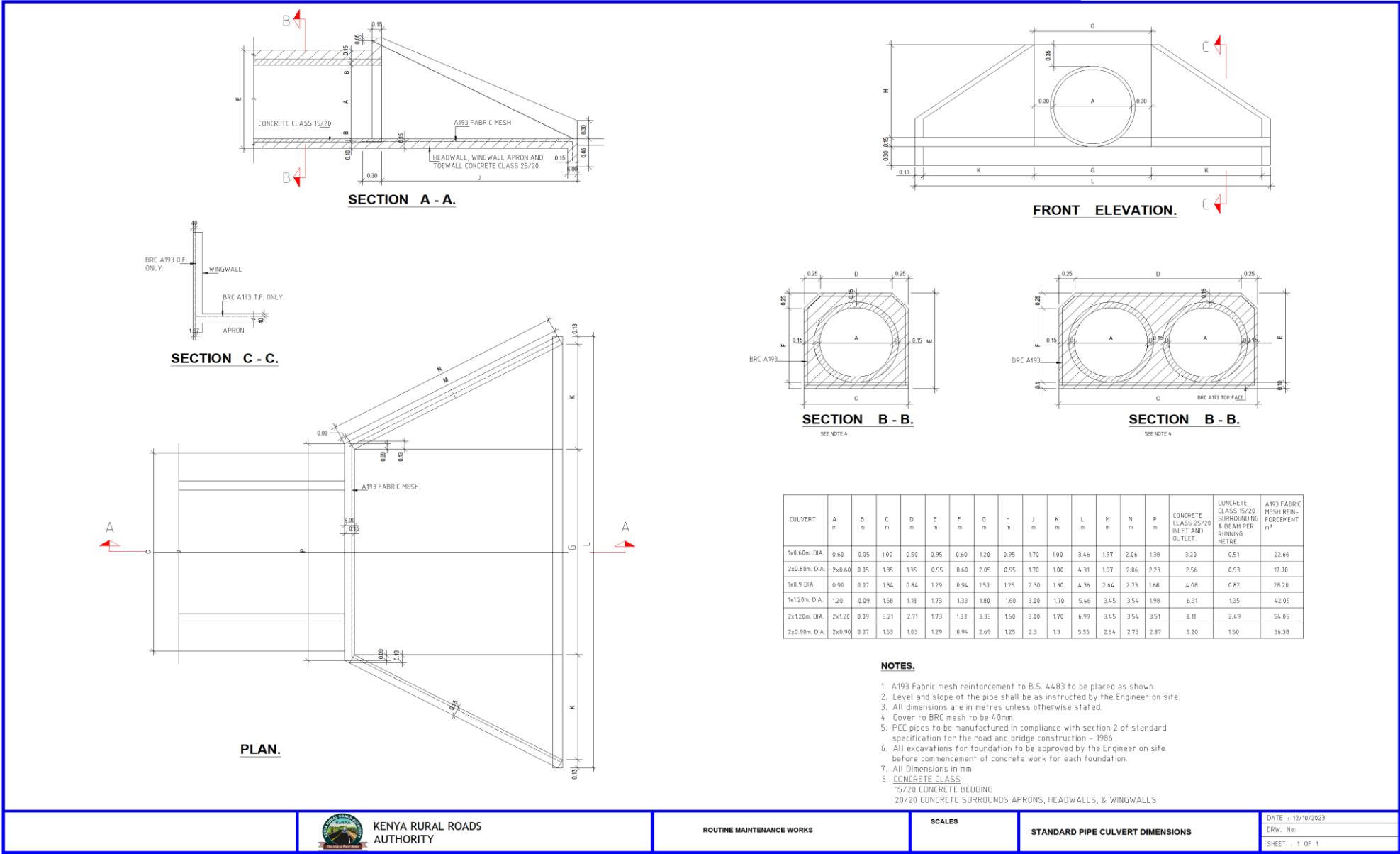
Fig. C.8 Standard pipe culvert Dimensions (900mm &600mm Diameter)
