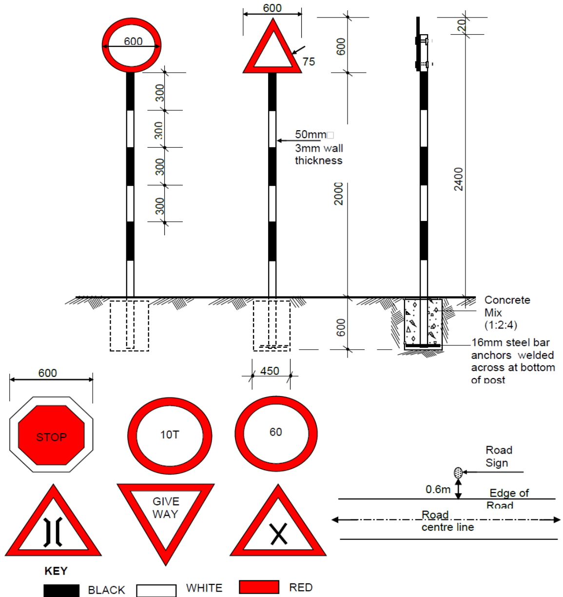
FIGURE C.16 - TRAFFIC SIGNS
