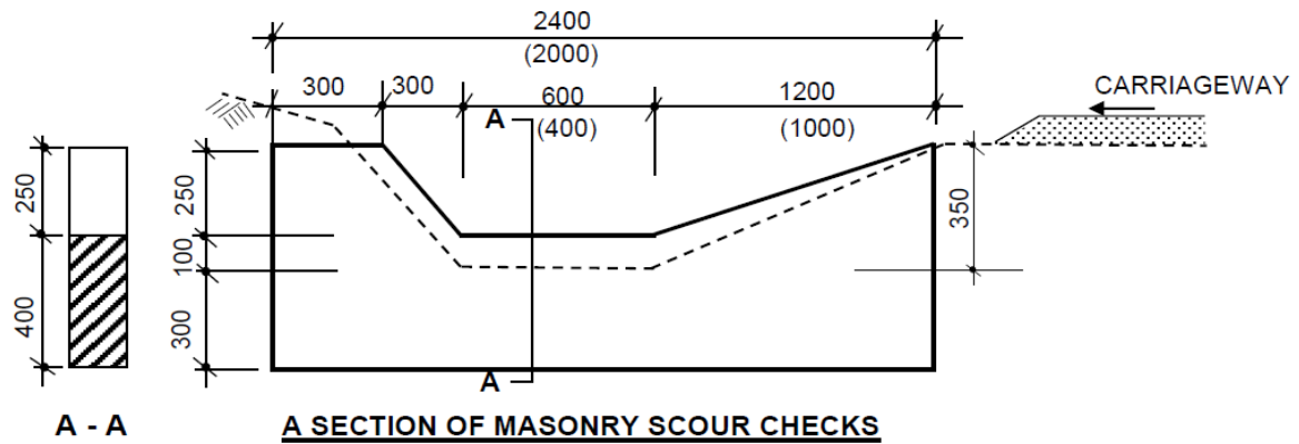
FIGURE C.6 - MASONRY SCOUR CHECKS
