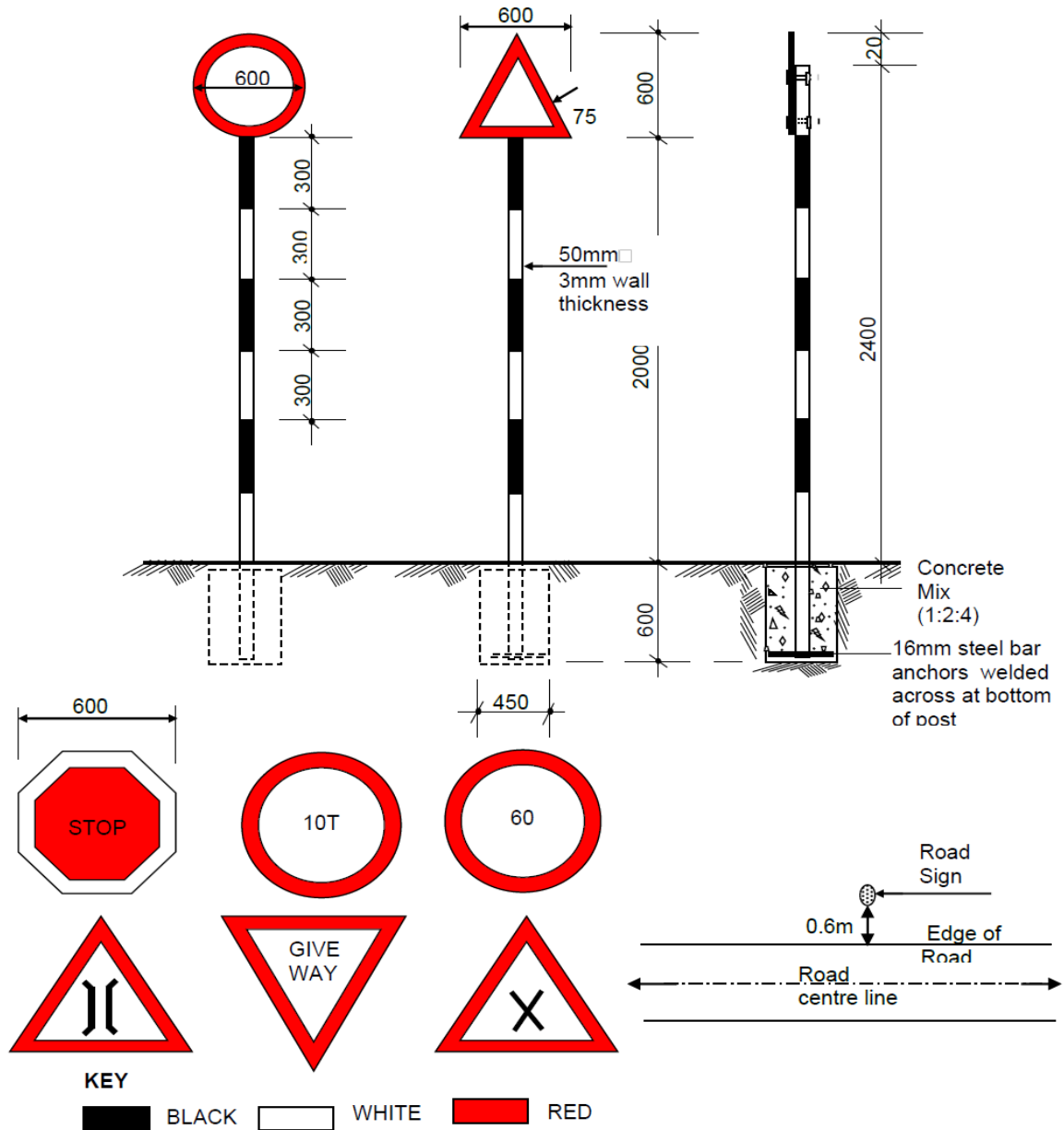
FIGURE C.16 - TRAFFIC SIGNS
