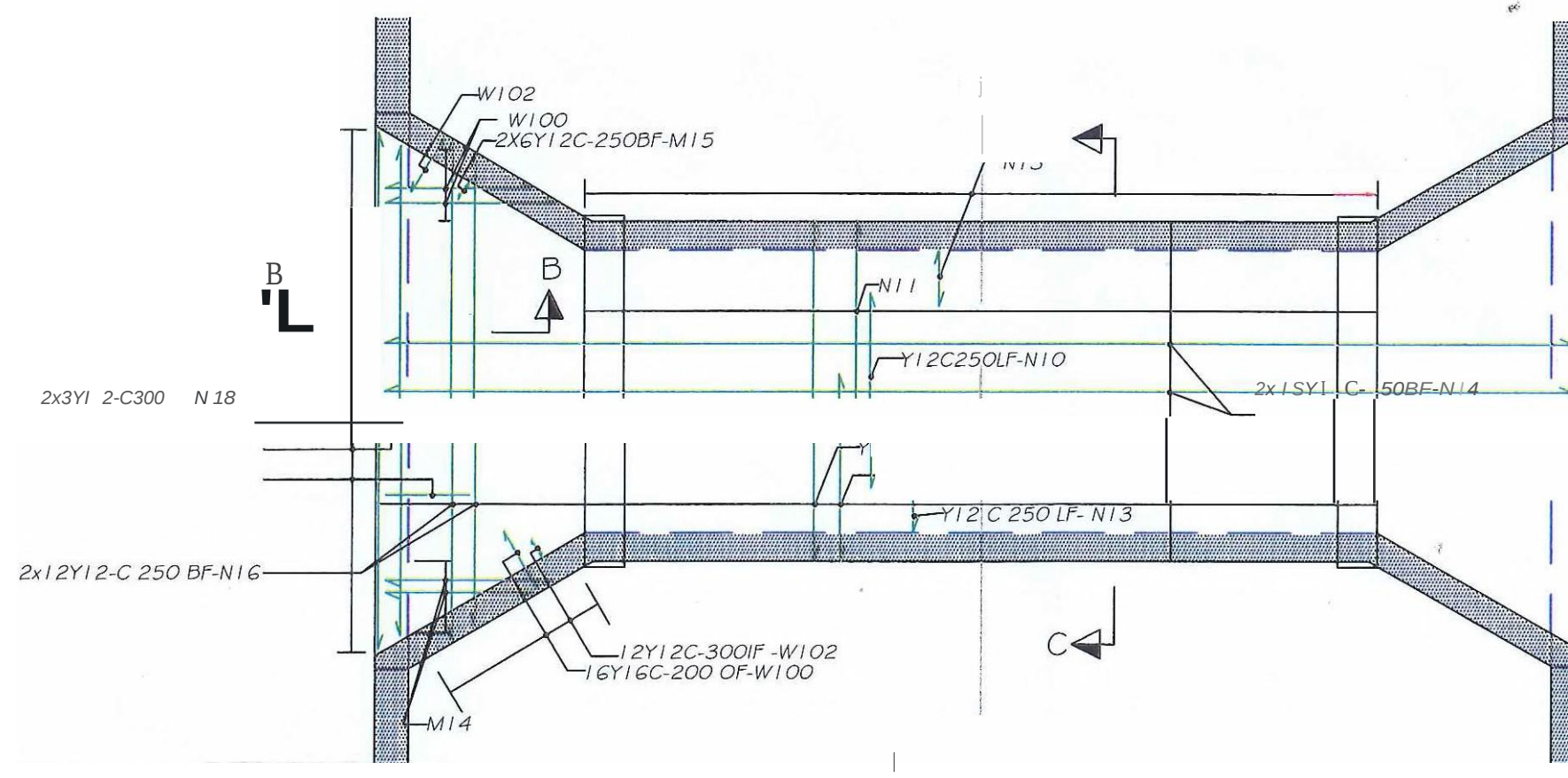
TOP SLAB REINFORCEMENT
