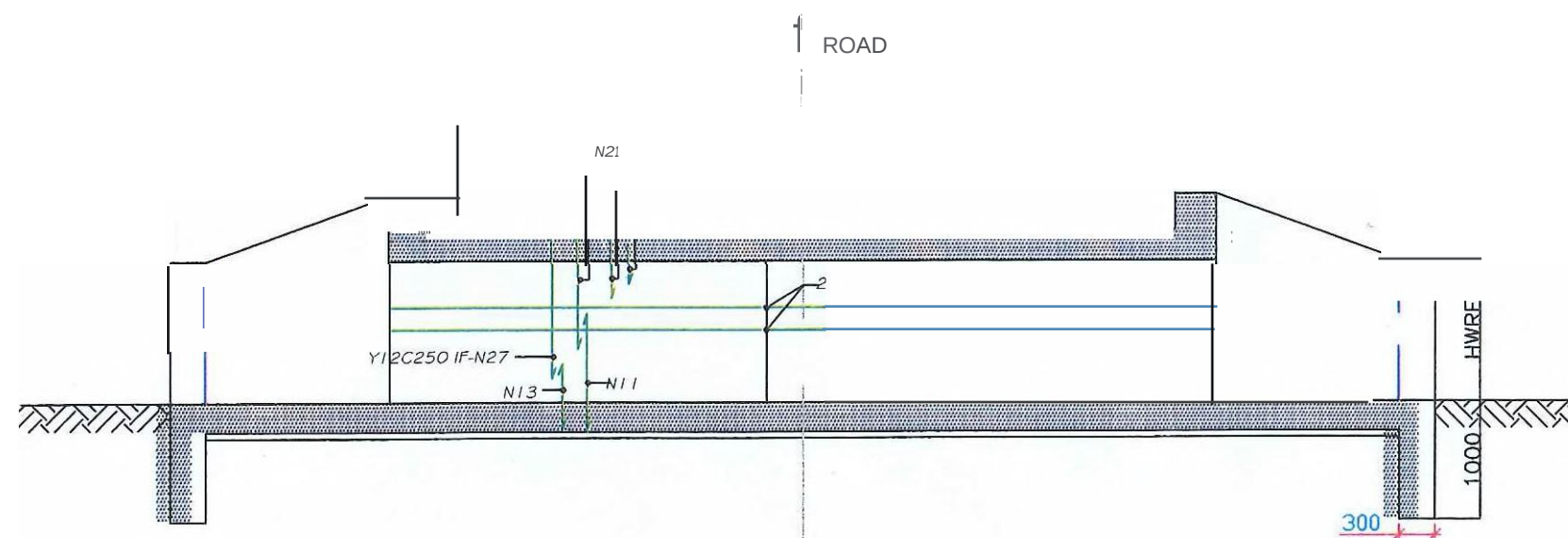
Elevation of outer and wingwalls
