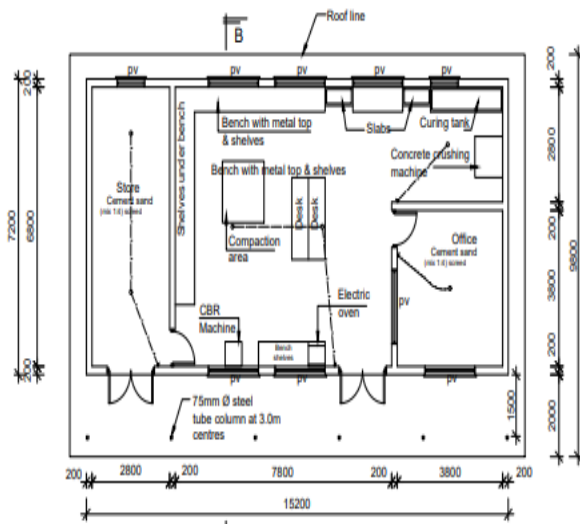
Soils Laboratory-Plan Scale 1:125
