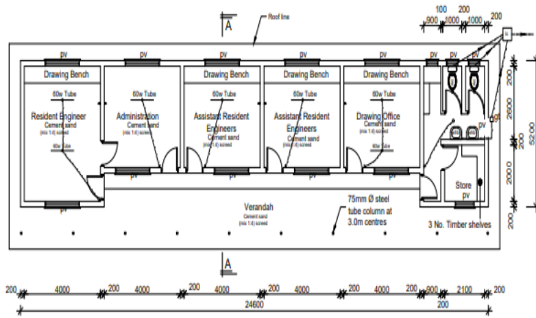
Resident Engineers Site Office-Plan Scale 1:125
