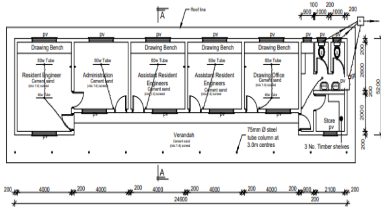
Resident Engineers Site Office-Plan Scale 1:125
