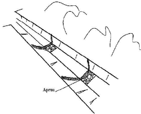
Scour checks made of wooden stakes
