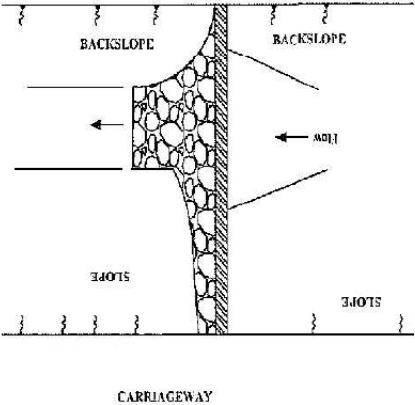
SECTION OF CONCRETE SCOUR CHECK
