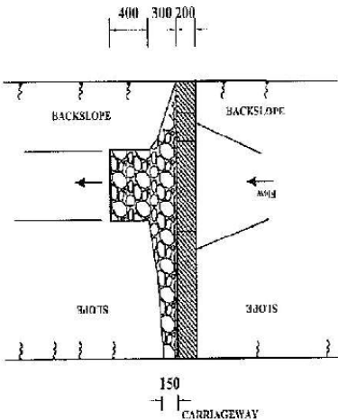
PLAN OF DRAIN WITH SCOUR CHECK
