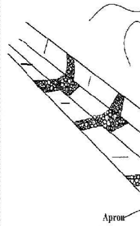
Scour checks made of stones
