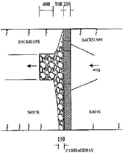
PLAN OF DRAIN WITH SCOUR CHECK
