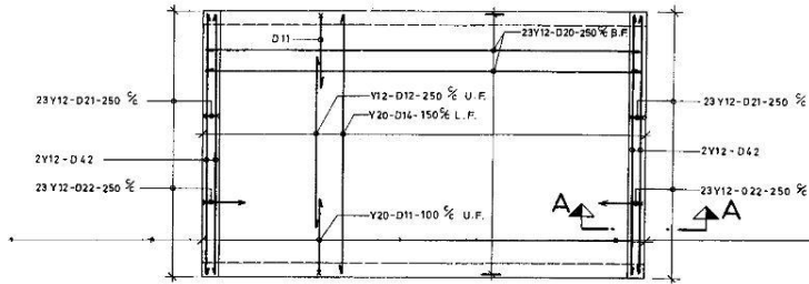
PLAN OF TOP SLAB. SCALE 1:50
