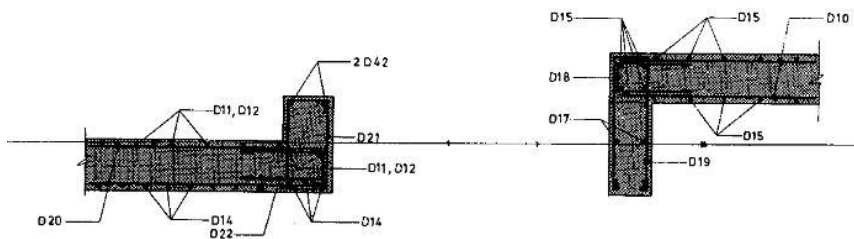
SECTION A. SCALE 1:20
