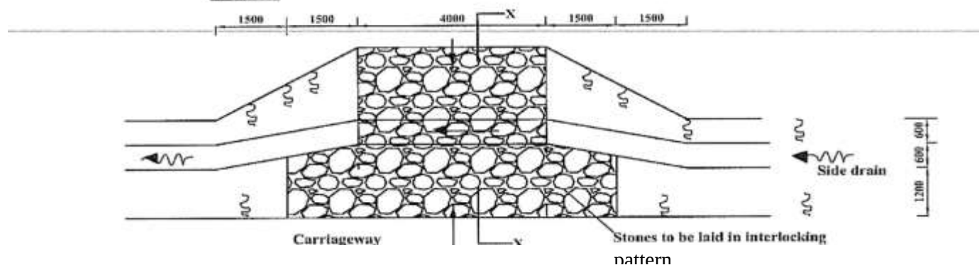
FIGURE C18-ACCESS DRIFT
