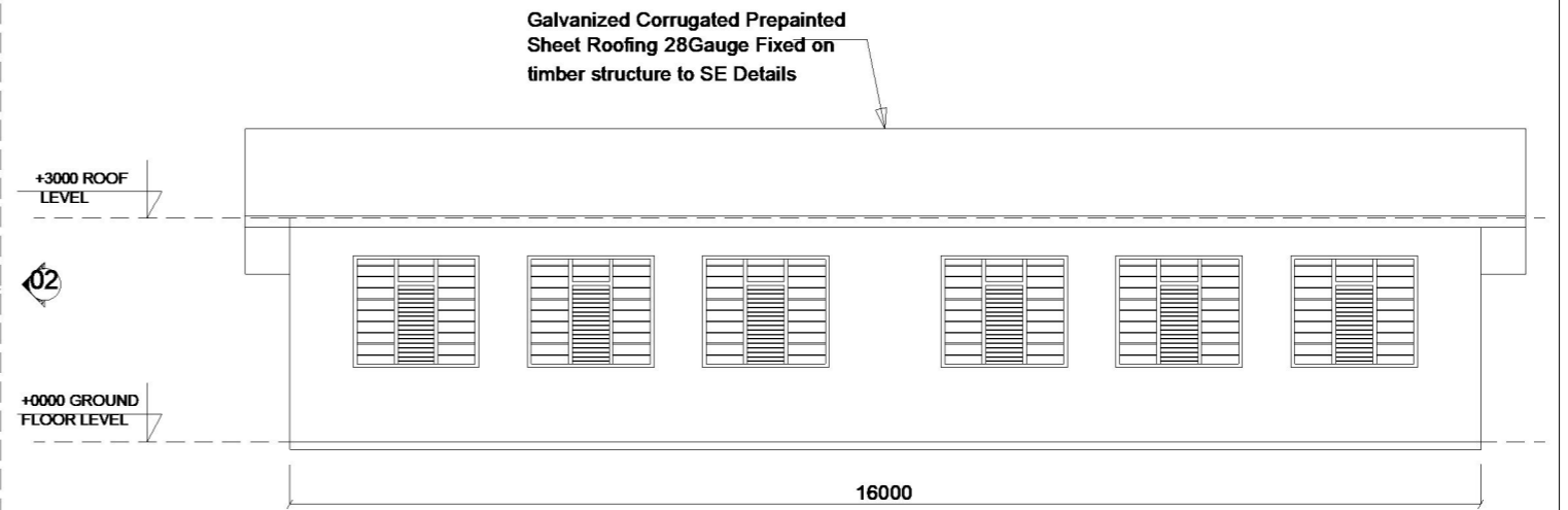
ELEVATION 03
