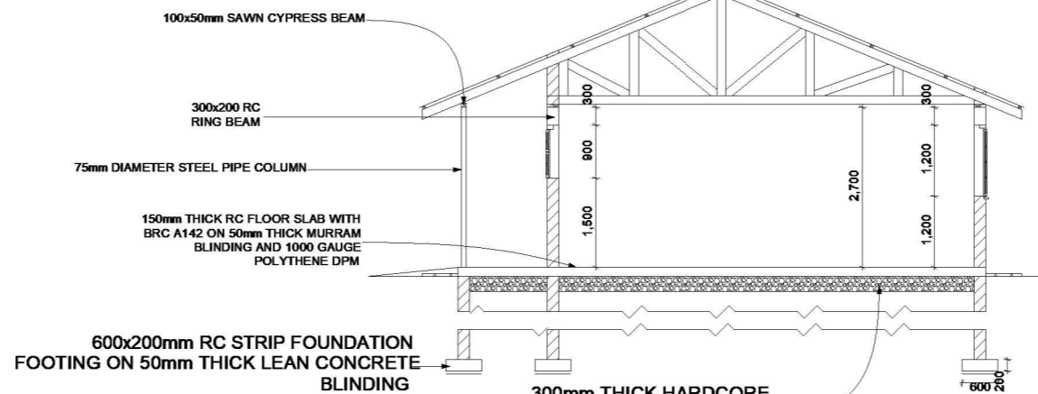
SECTION 01-01
