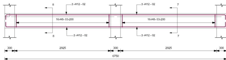
Beam GB2 Elevation
