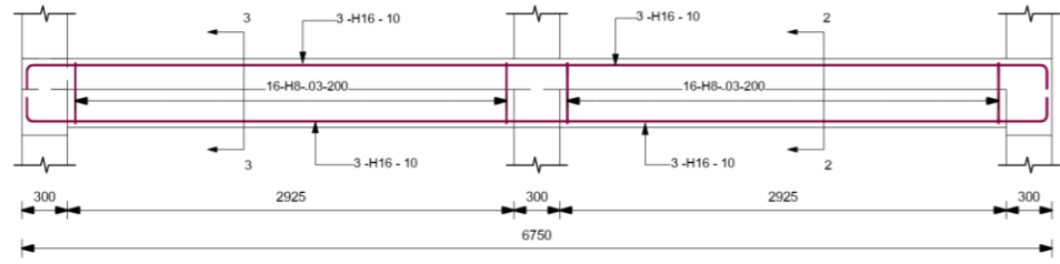
Beam TB2 Elevation 1 : 25
