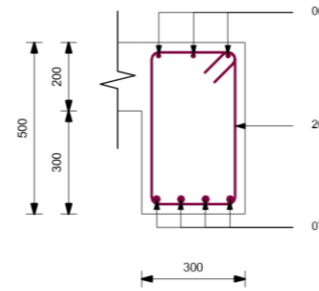
TB1 Section 11-11
