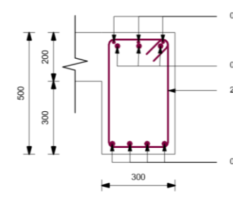
TB1 Section 12-12
