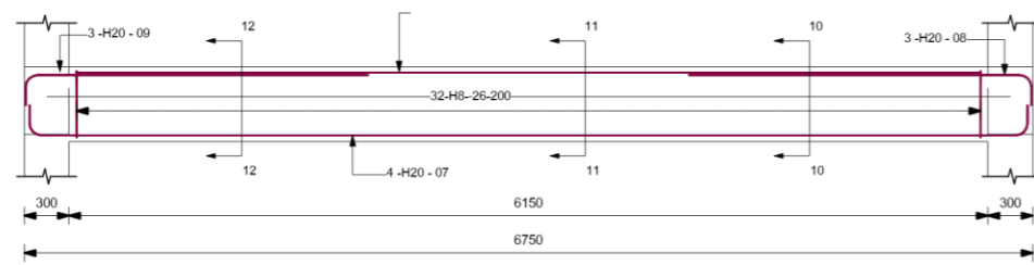
Beam TB1 Elevation
