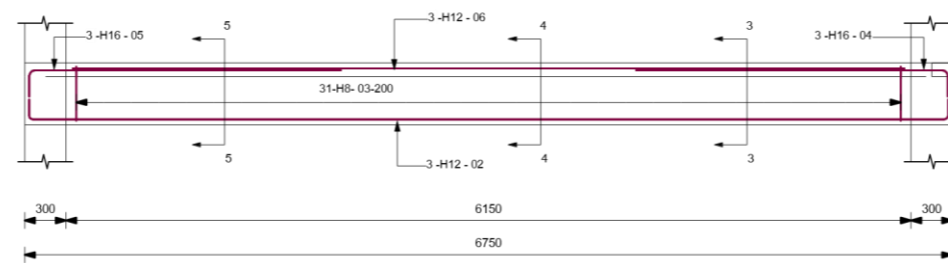
Beam GB1 Elevation
