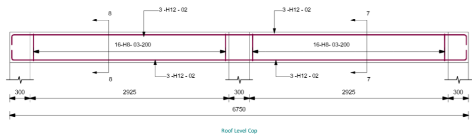
Beam RB2 Elevation 1 : 25
