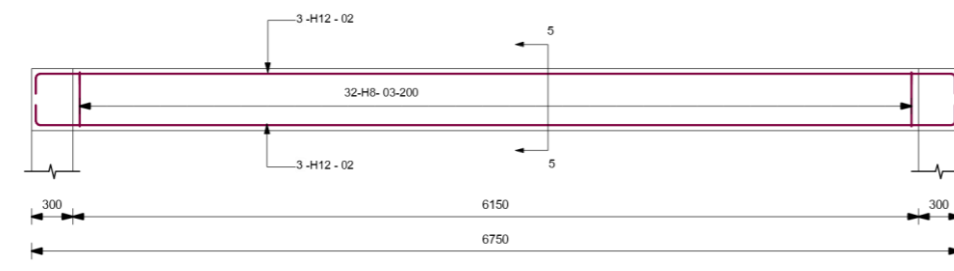
Beam RB1 Elevation 1 : 25
