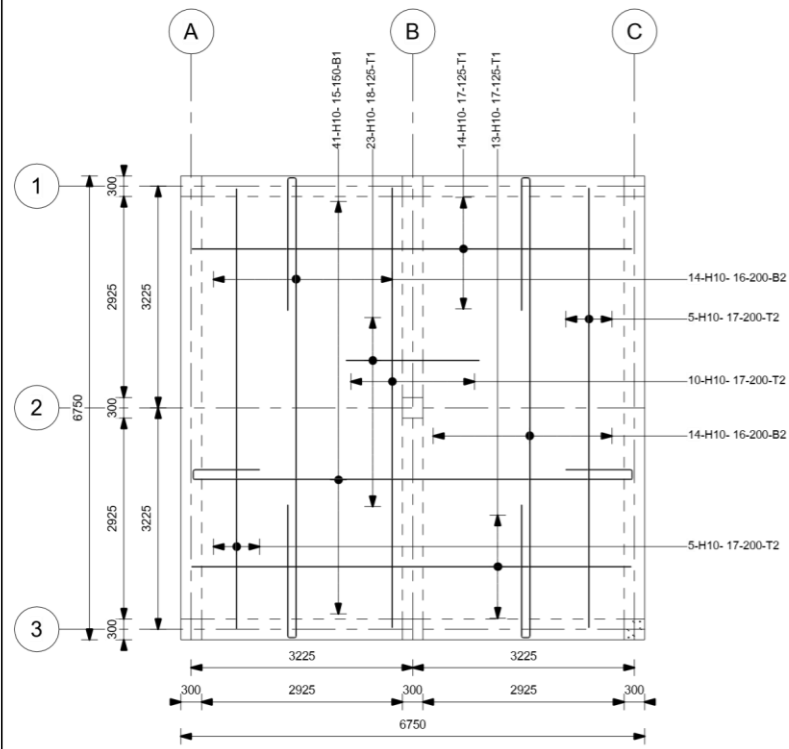
Typical Floor
