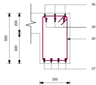
TB1 Section 10-10
