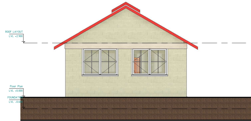
① SIDE ELEVATION A 1 : 50
