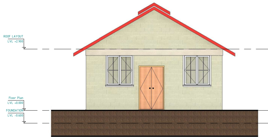
③ SIDE ELEVATION B 1 : 50
