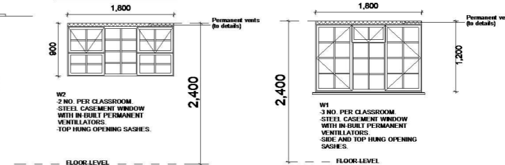
WINDOW SCHEDULE
