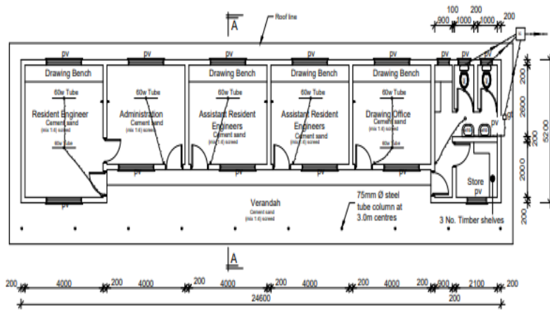
Resident Engineers Site Office-Plan Scale 1:125
