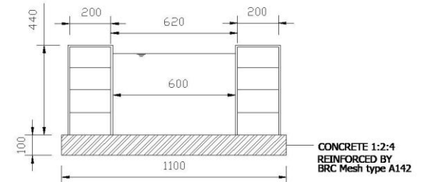
SECTION G-G
