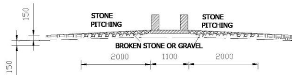
SECTION B-B
