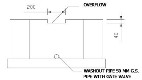
FRONT VIEW SECTION H-H
