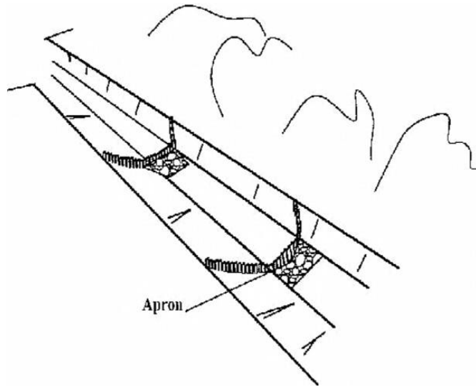
Scour checks mat!~ of wood~n sl~kes
